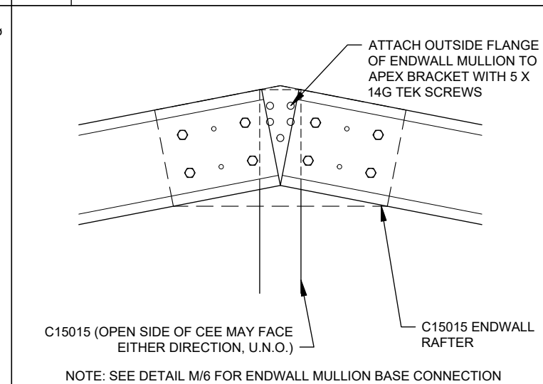
C2 ENDWALL MULLION TO RAFTER PEAK CONDITION
