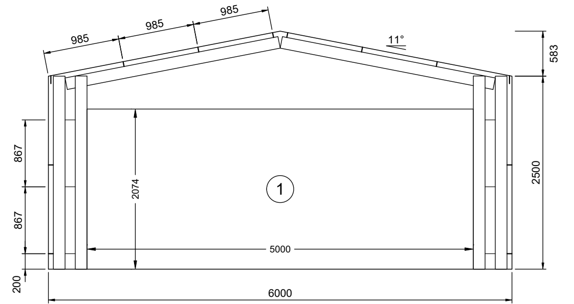
4 FRONT ELEVATION 3 SCALE: 1:50 FRAME #1
