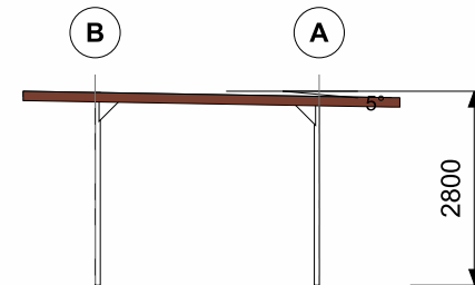
ELEVATION GRID 2
