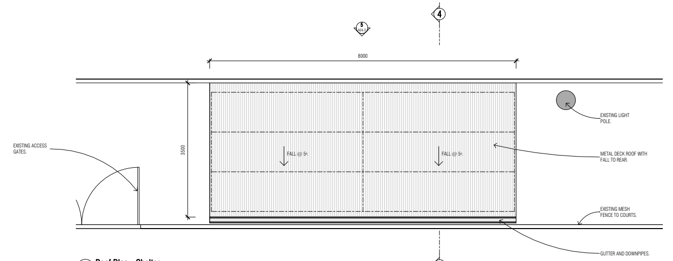
3 Roof Plan - Shelter 1:50
