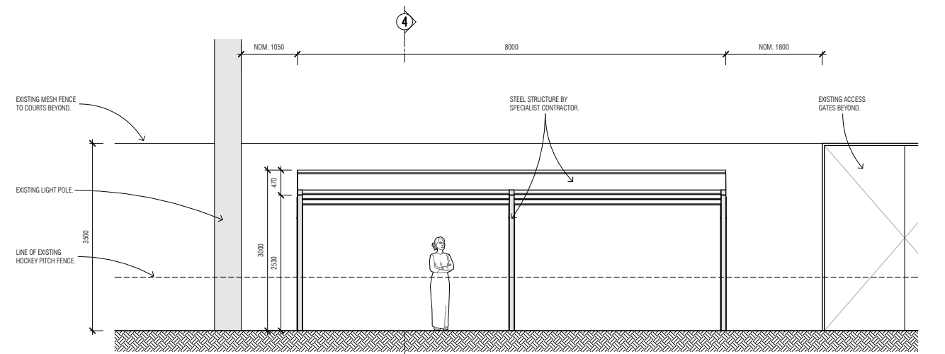
5 Elevation - Shelter 1:50
