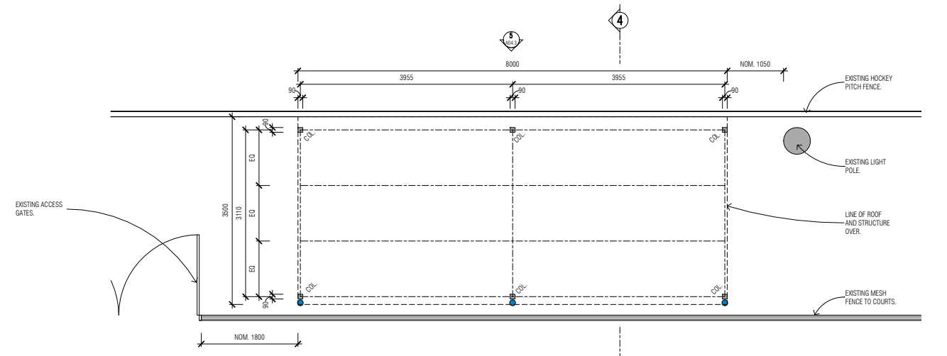
2 Ground Floor Plan - Shelter 1:50
