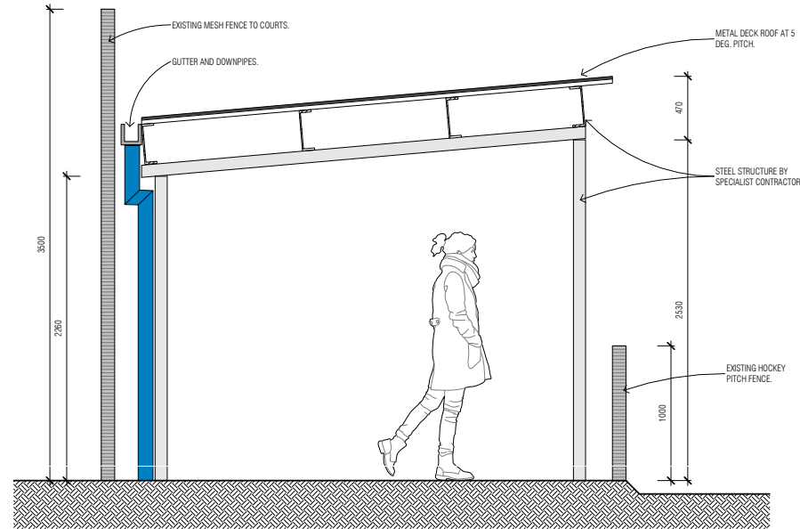
4 Section - Shelter 1:25
