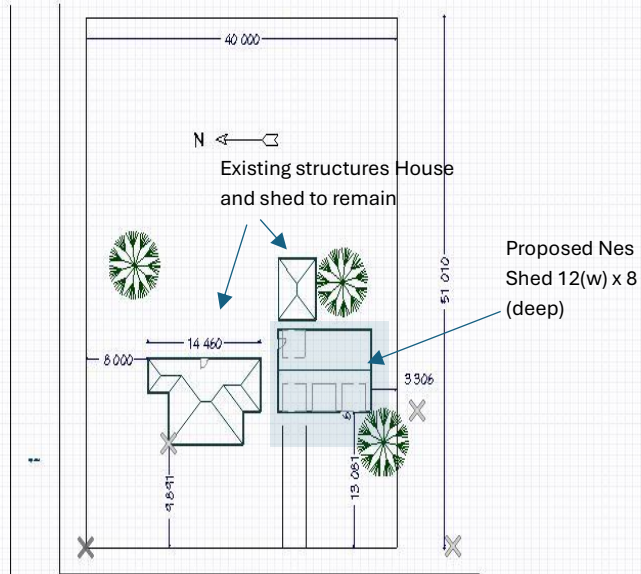
Site Plan
