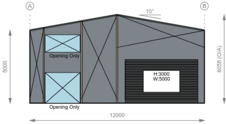
End Wall 1
