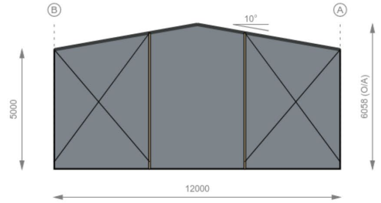
End Wall 5
