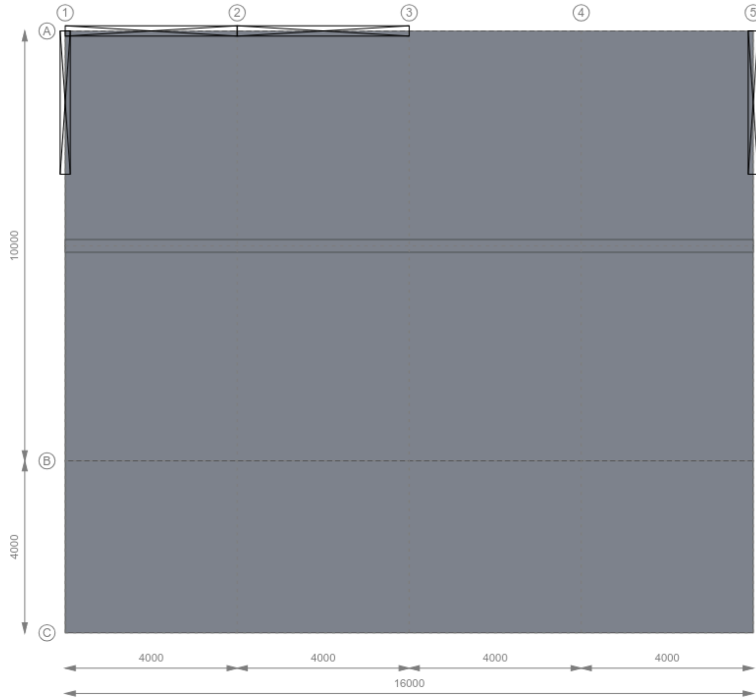
Roof plan
