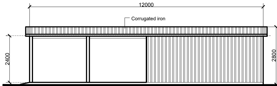
EAST ELEVATION
