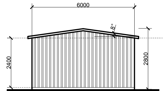
NORTH ELEVATION
