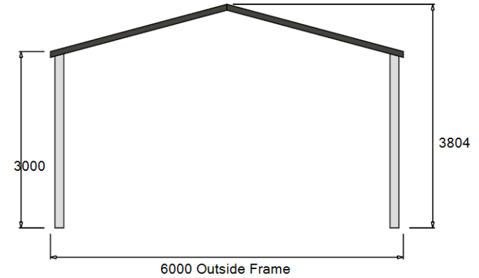
Front Internal Elevation - 3
