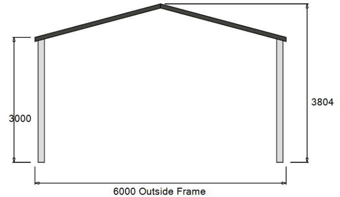
Rear Internal Elevation - 1
