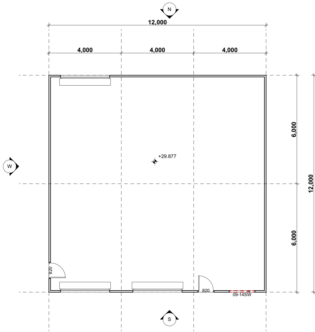
GROUND
