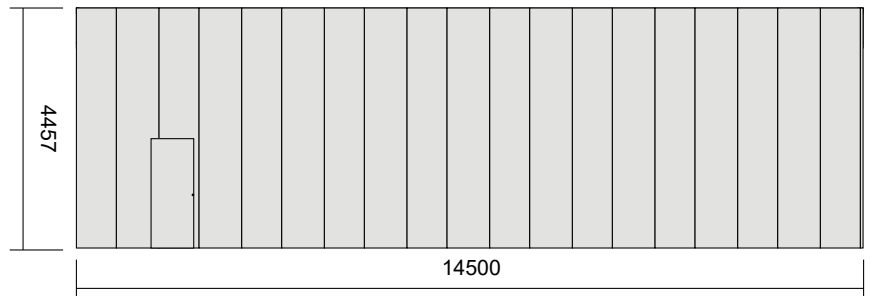
High Side Elevation
