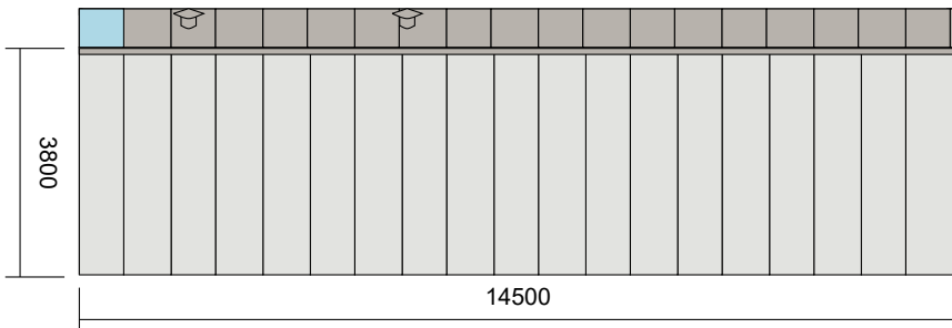
Low Side Elevation
