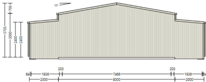
Right Elevation (1:99)
