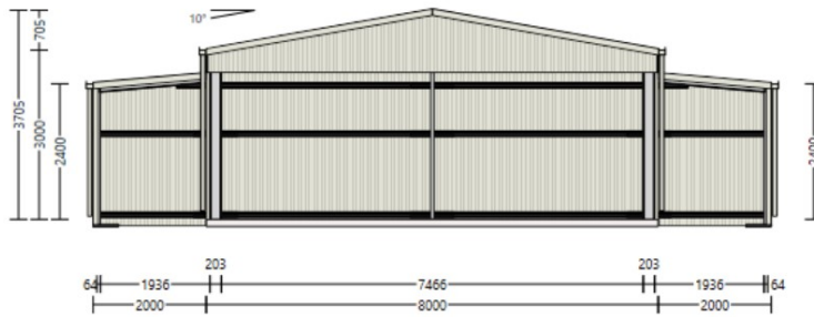
Left Elevation (1:99)
