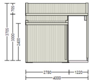
Rear Elevation (1:99)
