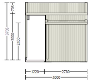
Front Elevation (1:99)
