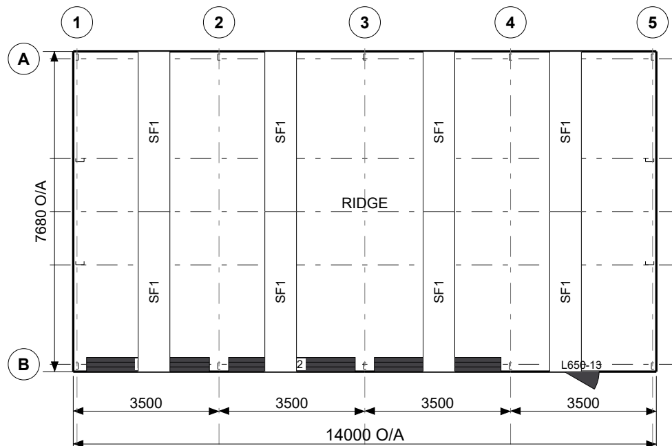
FRAME ROOF PLAN
