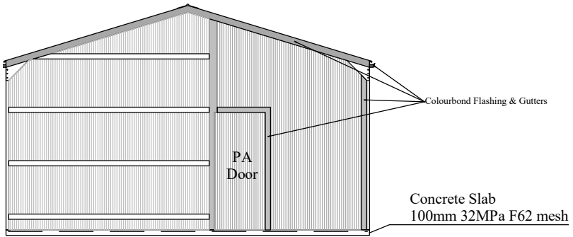
SW External Elevation
