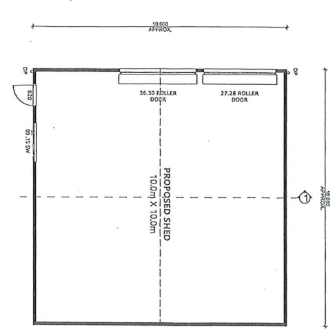
SHED FLOOR PLAN SCALE: 1:100
