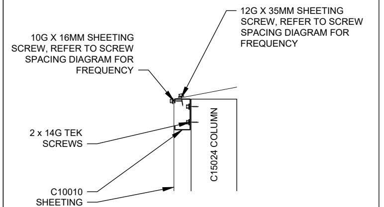
I WALL SHEETING
