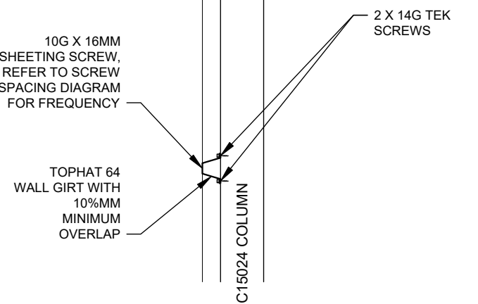
F GIRTS CONNECTION
