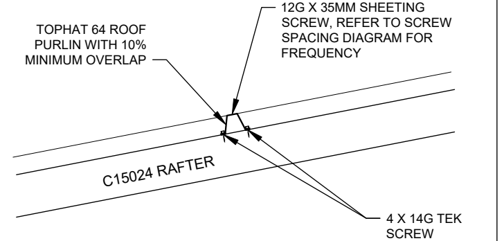
G EAVE CONNECTION
