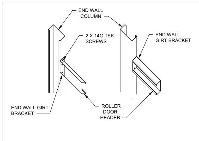
N END DOOR HEADER AND JAMB
