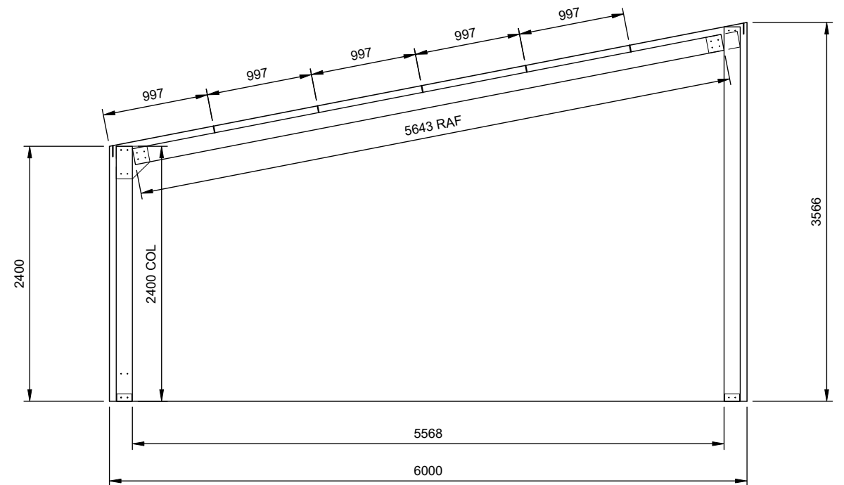
1 ROOF ONLY FRAME CROSS-SECTION 8 SCALE: 1:50 FRAME 1
