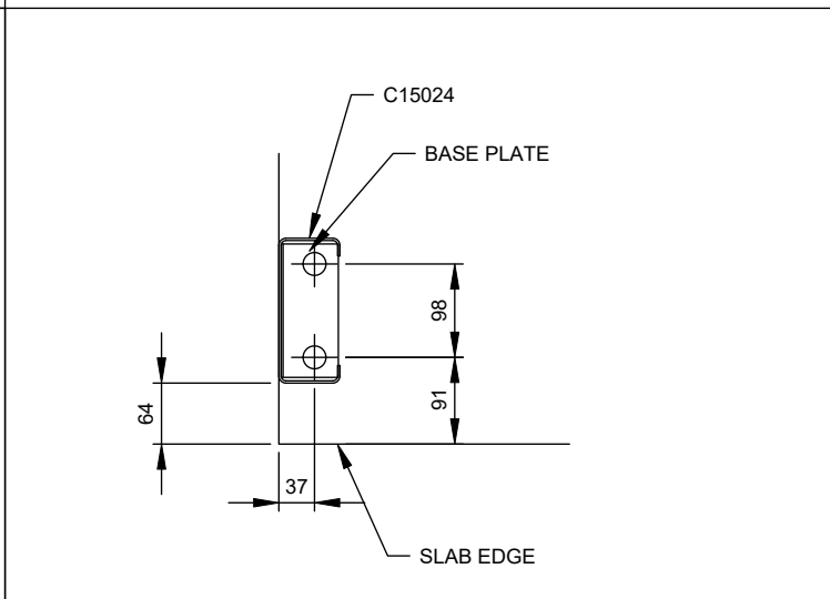
K ROOF ONLY COLUMN BASE
