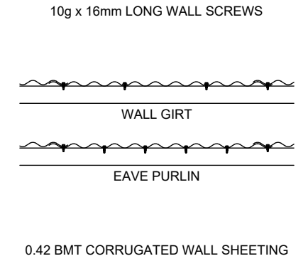
I WALL SHEETING
