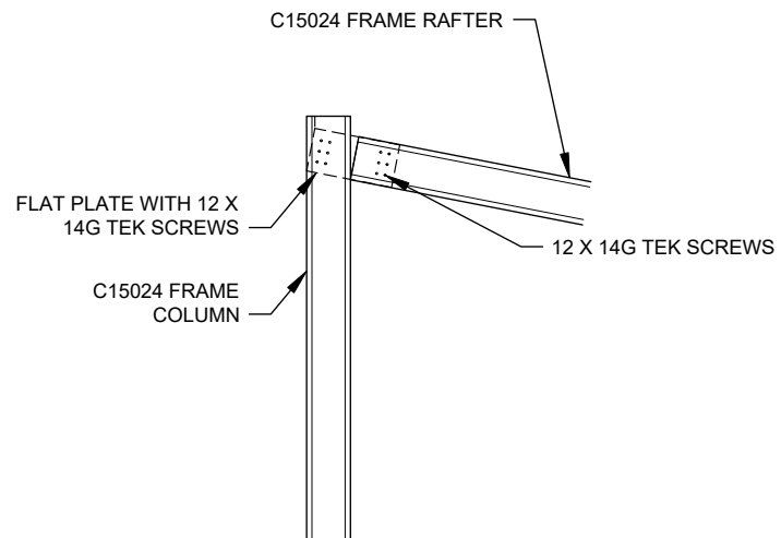
B HIGH EAVE HAUNCH CONNECTION
