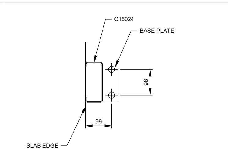
L ROTATED ENDWALL MULLION BASE
