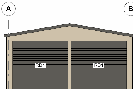
ELEVATION GRID 1
