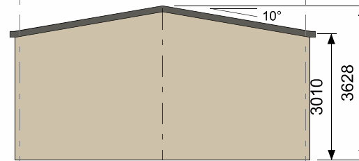
ELEVATION GRID 4
