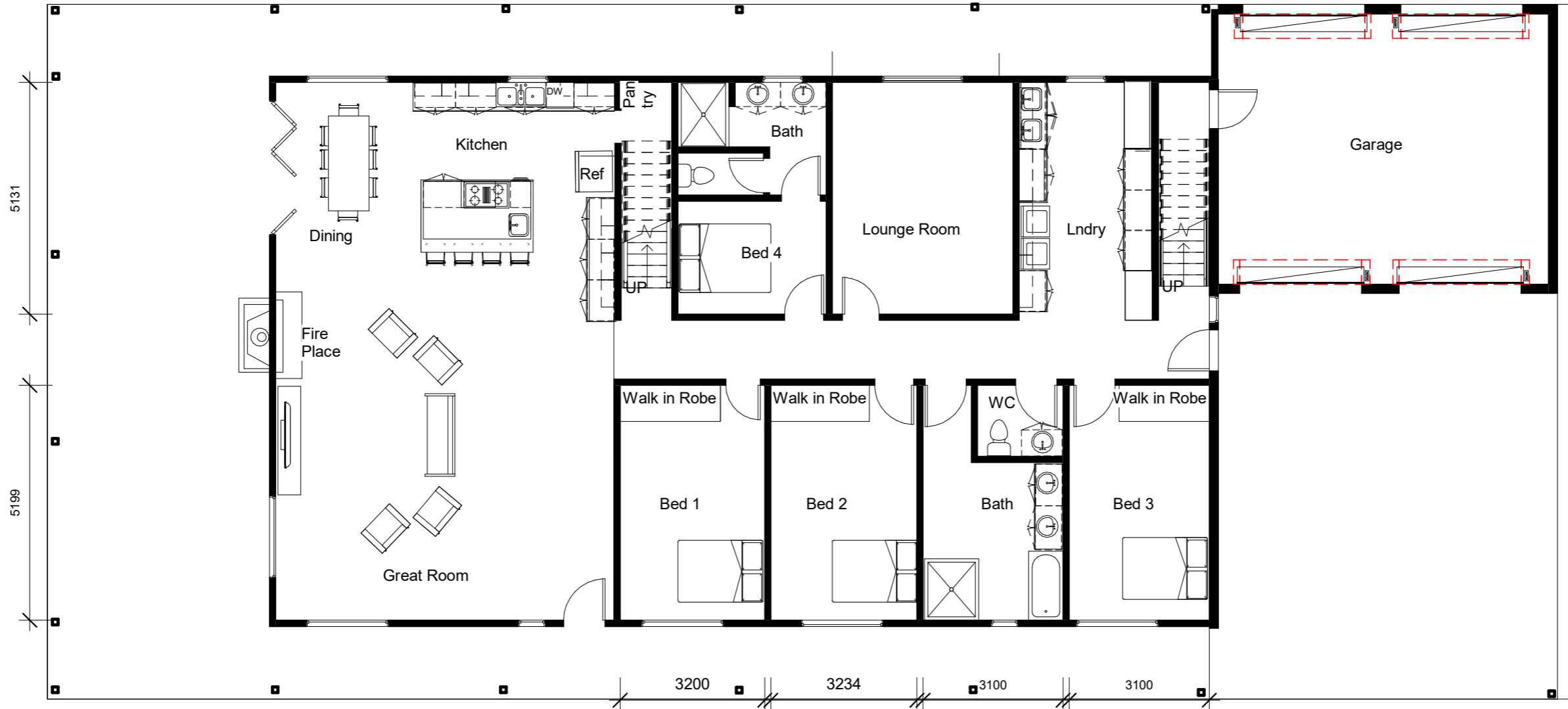
1 Level 1 1 to 100 1 : 100
