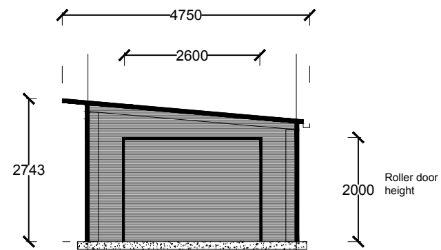
Rear Elevation
