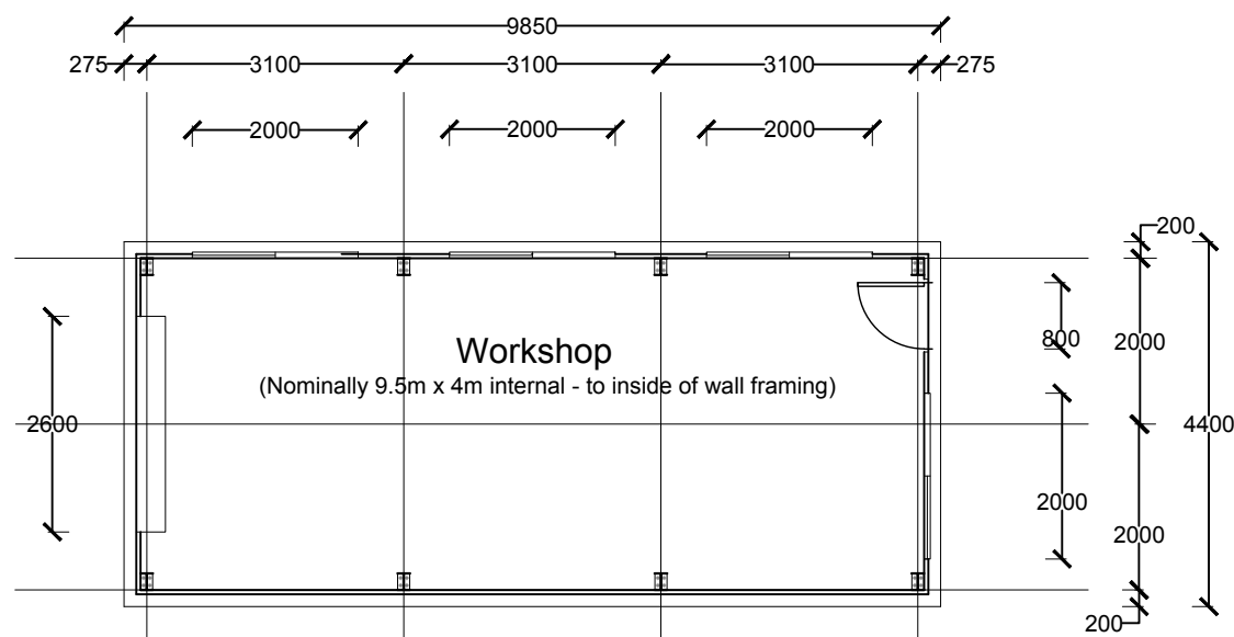
Ground Plan
