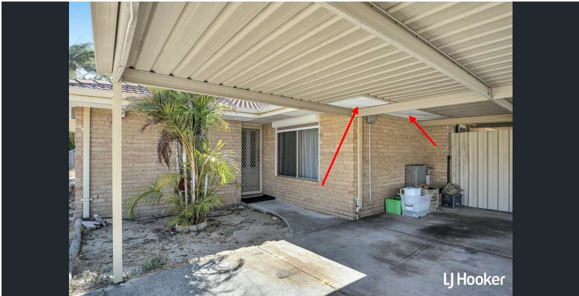
Figure 5 These arrows show where the roof gets on the way of the new design and installation and where some L-shaped structures need to be bolted into the external wall and wrap around the roof and protrude up to be the resting structure for the highest side of the skillion roof.
