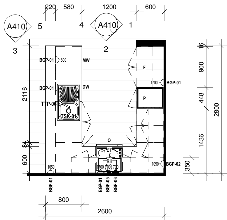
A KITCHEN PLAN 1 : 50
