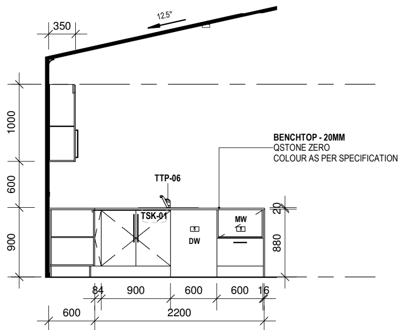
4 KITCHEN ELEVATION 4 1 : 50
