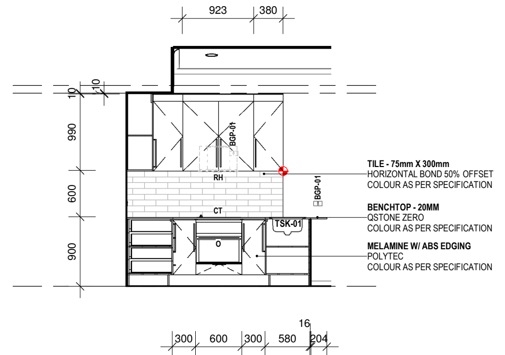
2 KITCHEN ELEVATION 2 1 : 50
