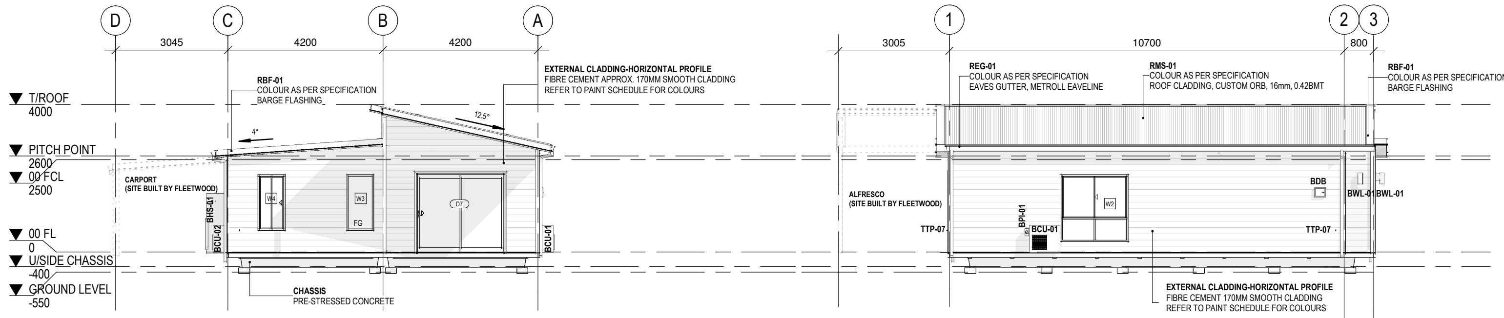
3 REAR ELEVATION 1 : 100
