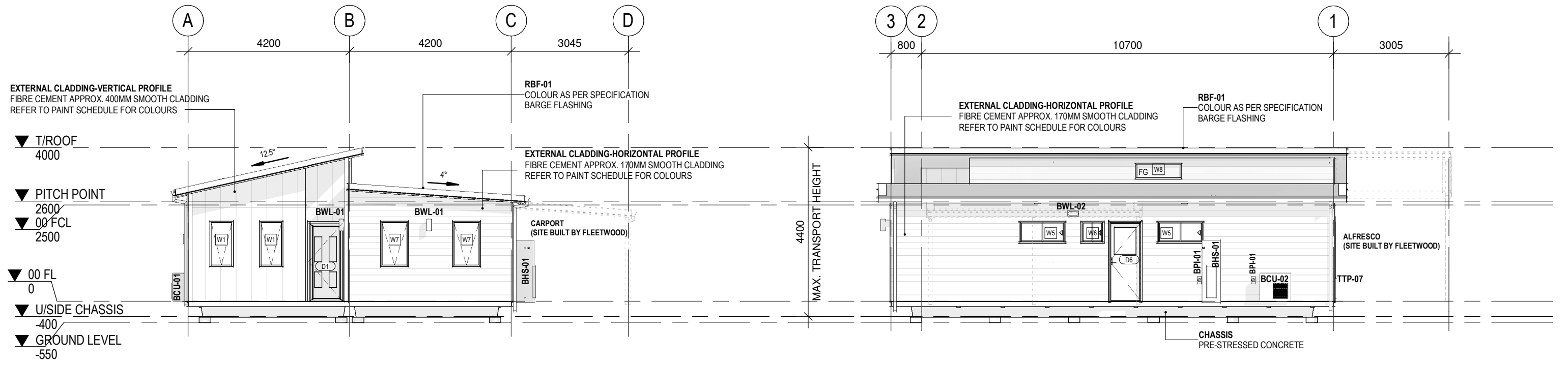
1 FRONT ELEVATION 1 : 100
