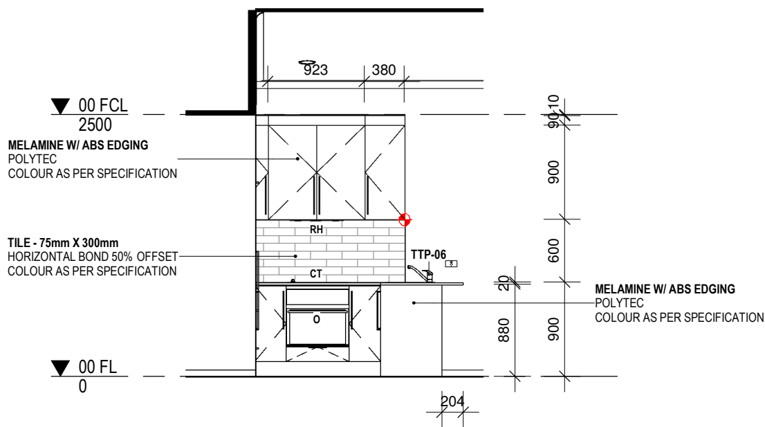
3 KITCHEN ELEVATION 3 1 : 50
