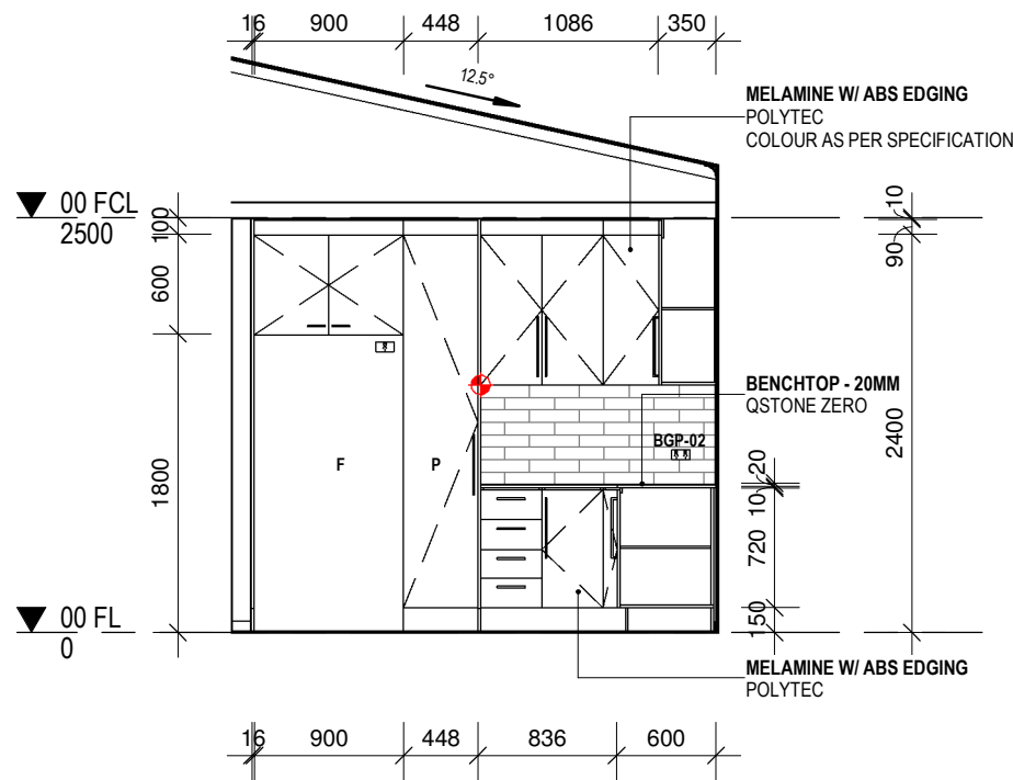
1 KITCHEN ELEVATION 1 1 : 50
