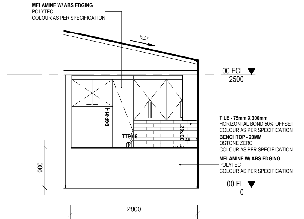
5 KITCHEN ELEVATION 5 1 : 50
