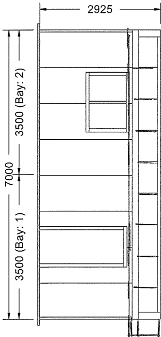
LEFT ELEVATION
