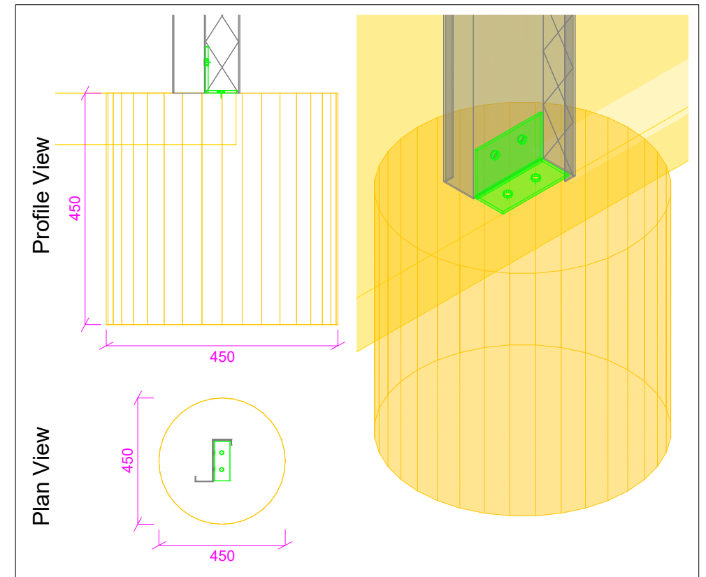
Footing: F3 (x2)
