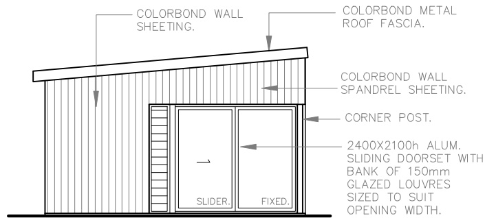
Elevation 2 - north
