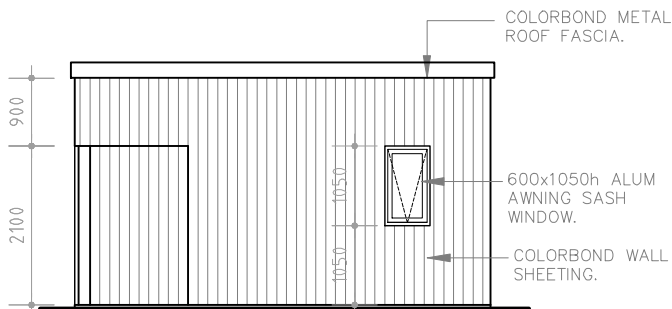
Elevation 3 - west
