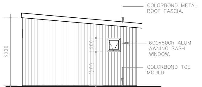
Elevation 4 - south
