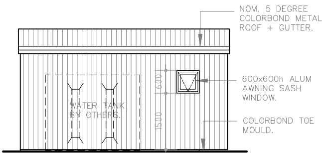
Elevation 1 - east
