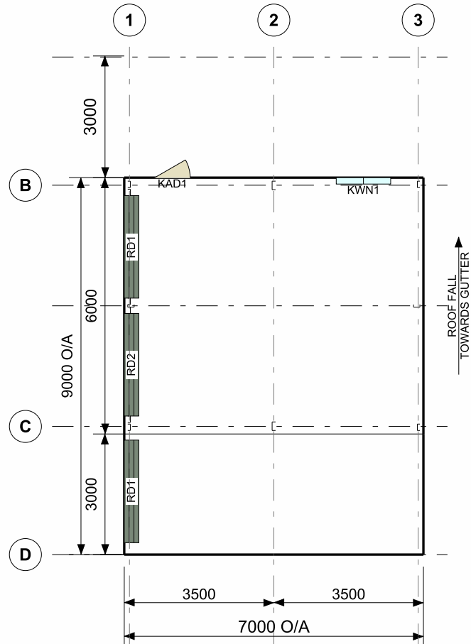
FRAME ROOF PLAN
