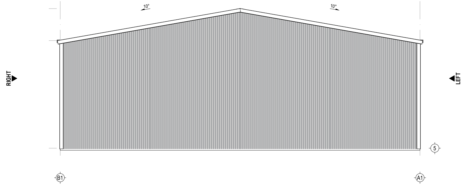
REAR ELEVATION
