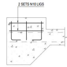
PLINTH (P1) (4 OFF) SCALE 1:10
