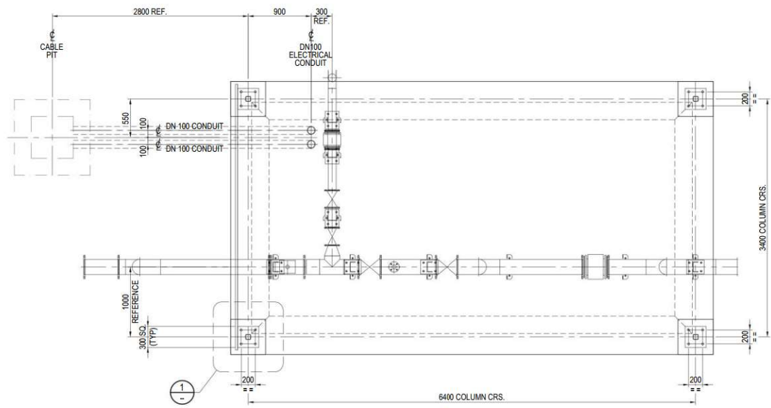
PLAN SCALE 1:25
