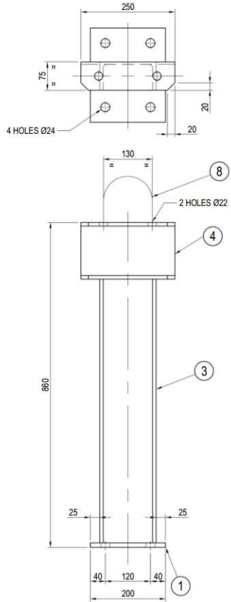
PIPE SUPPORT PS3 -3 REQ'D. SCALE 1:5
