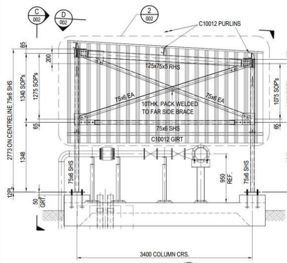
DETAIL 1 SCALE 1:10
