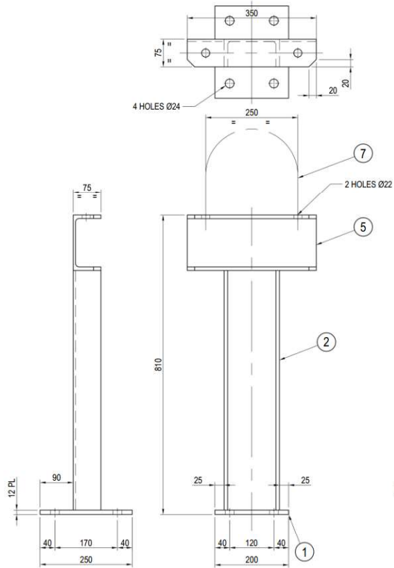
PIPE SUPPORT PS2 -4 REQ'D. SCALE 1:5
