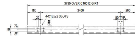
GIRT DETAILS (1 REQUIRED)
