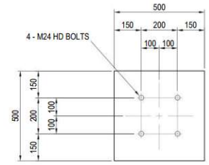
PLAN ON PLINTH (P1)
