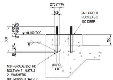
PLINTH (P1) (4 OFF) SCALE 1:10
