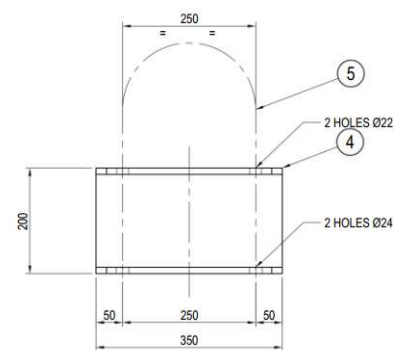
PIPE SUPPORT PS4 -2 REQD. SCALE 1:5
