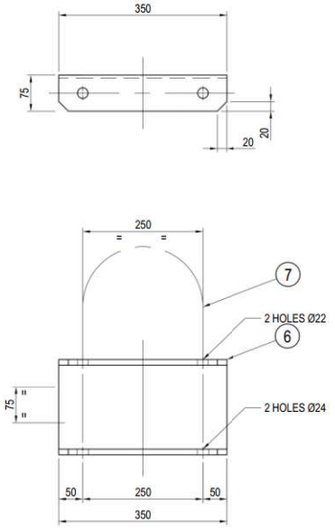
PIPE SUPPORT PS4 -2 REQ'D. SCALE 1:5
