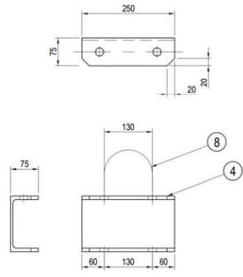
PIPE SUPPORT PS5 -1 REQ'D. SCALE 1:5
