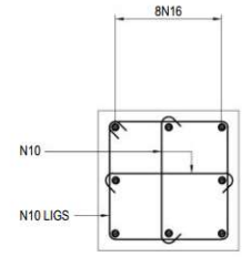
PLAN ON PLINTH (P1)
