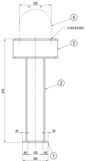
PIPE SUPPORT PS2 -3 REQD. SCALE 1:5
