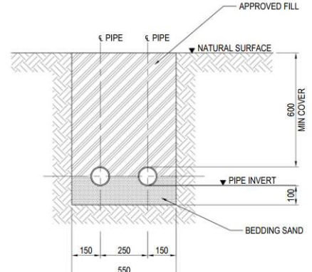
TYPICAL TRENCH DETAIL FOR 2x 100 LV & COMMS. CONDUITS SCALE 1:10
