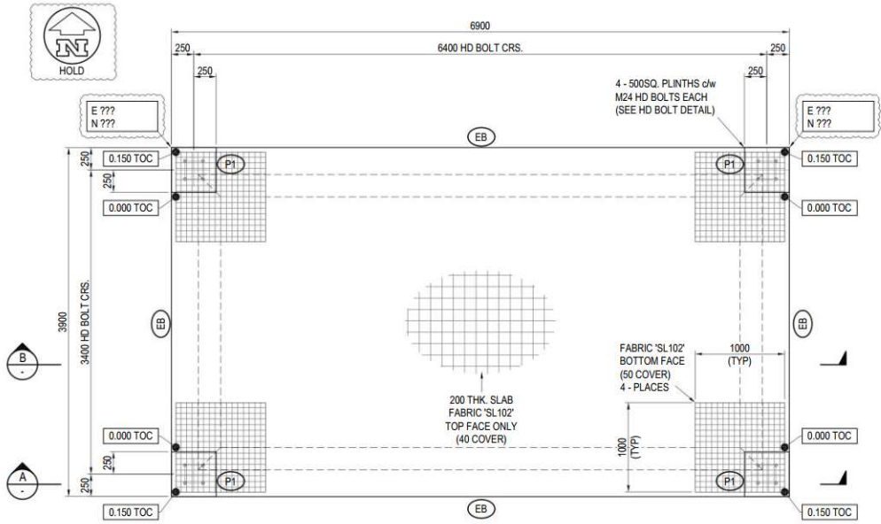
PLAN ON VALVE STATION SLAB (SCALE 1:25)
