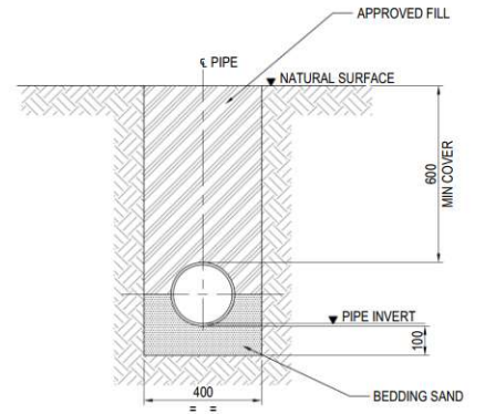
TYPICAL TRENCH DETAIL FOR DN200 SS PIPE SCALE 1:10
