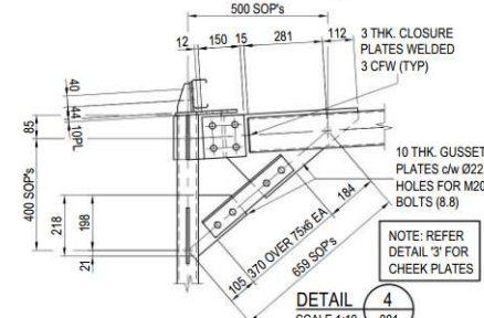
DETAIL 3 SCALE 1:10 001 & -
