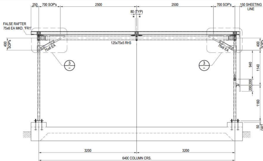
VIEW ON C SCALE 1:25 001
