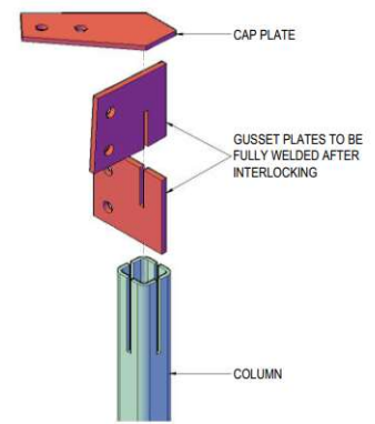
EXPLODED VIEW SHOWING CRUCIFORM ASSEMBLY (TYPICAL GUSSETS & CAP PLATE PER COLUMN)
