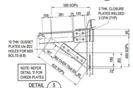
DETAIL 5 SCALE 1:10 001
