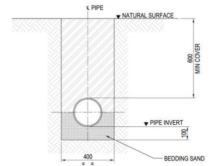
TYPICAL TRENCH DETAIL FOR DN200 SS PIPE SCALE 1:10
