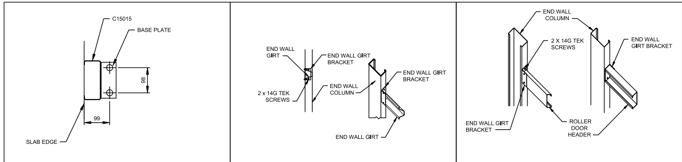
N ROTATED ENDWALL MULLION BASE O ENDWALL GIRT BRACKET P END DOOR HEADER AND JAMB
