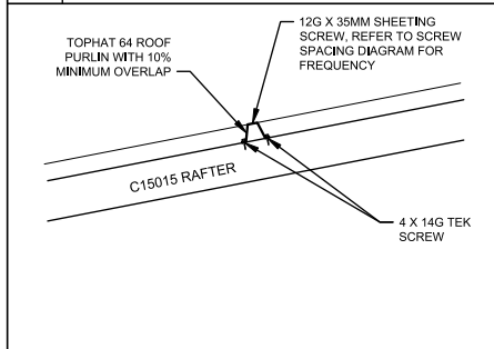
E PURLIN CONNECTION
