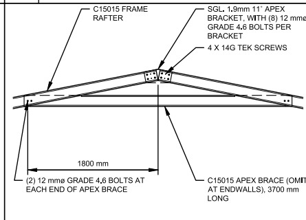
B APEX CONNECTION
