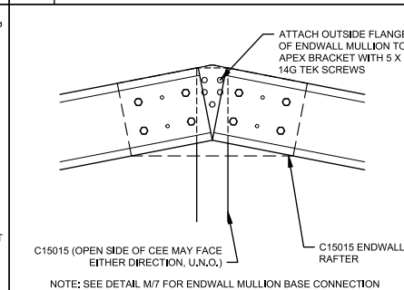
C2 ENDWALL MULLION TO RAFTER PEAK CONDITION
