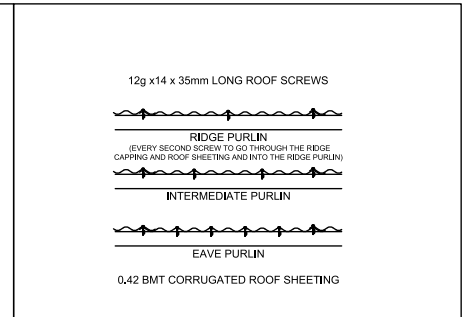
I ROOF SHEETING
