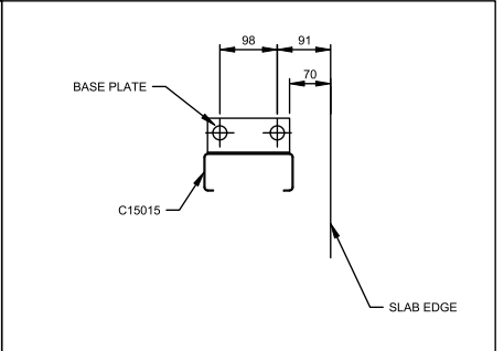
M ENDWALL MULLION BASE
