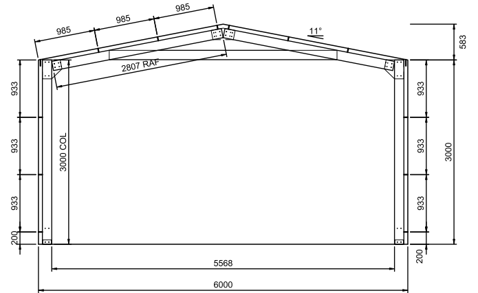
1 8 TYP. FRAME CROSS-SECTION SCALE: 1:50 FRAME 2
