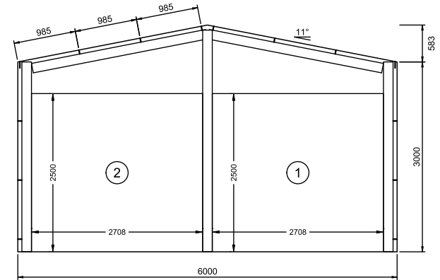
4 FRONT ELEVATION 4 SCALE: 1:50 FRAME #1
