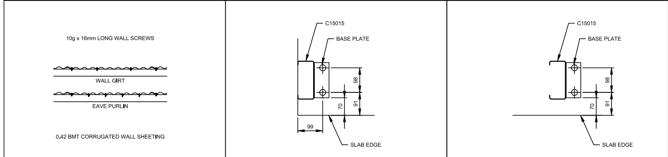
J WALL SHEETING K CORNER COLUMN BASE L INTERNAL COLUMN BASE
