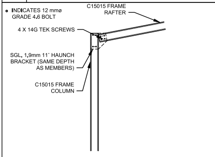
A HAUNCH CONNECTION
