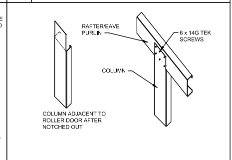
D ENDWALL MULLION ROTATED
