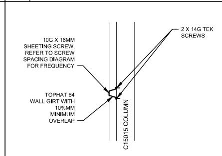
F GIRT CONNECTION
