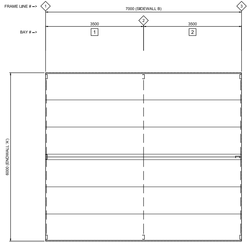
2 ROOF FRAMING PLAN 5 SCALE: 1:50
