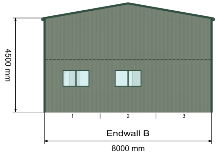
End Wall B
