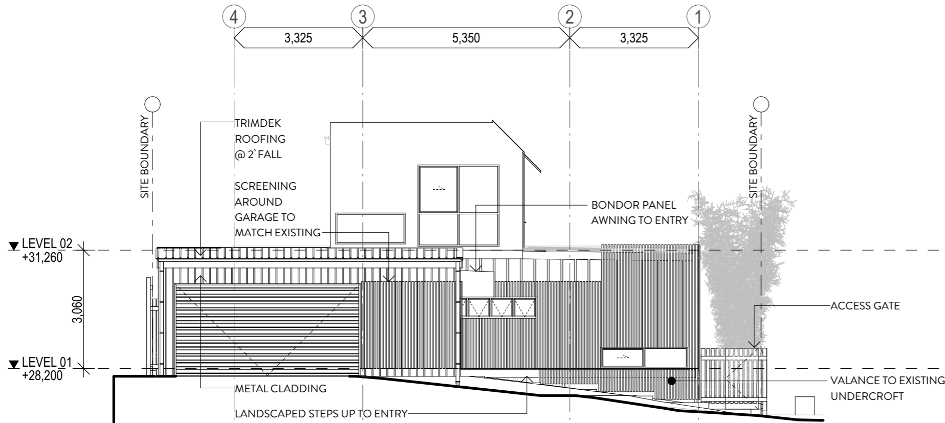
E-03 PROPOSED SOUTH ELEVATION SCALE 1:100 @ A3
