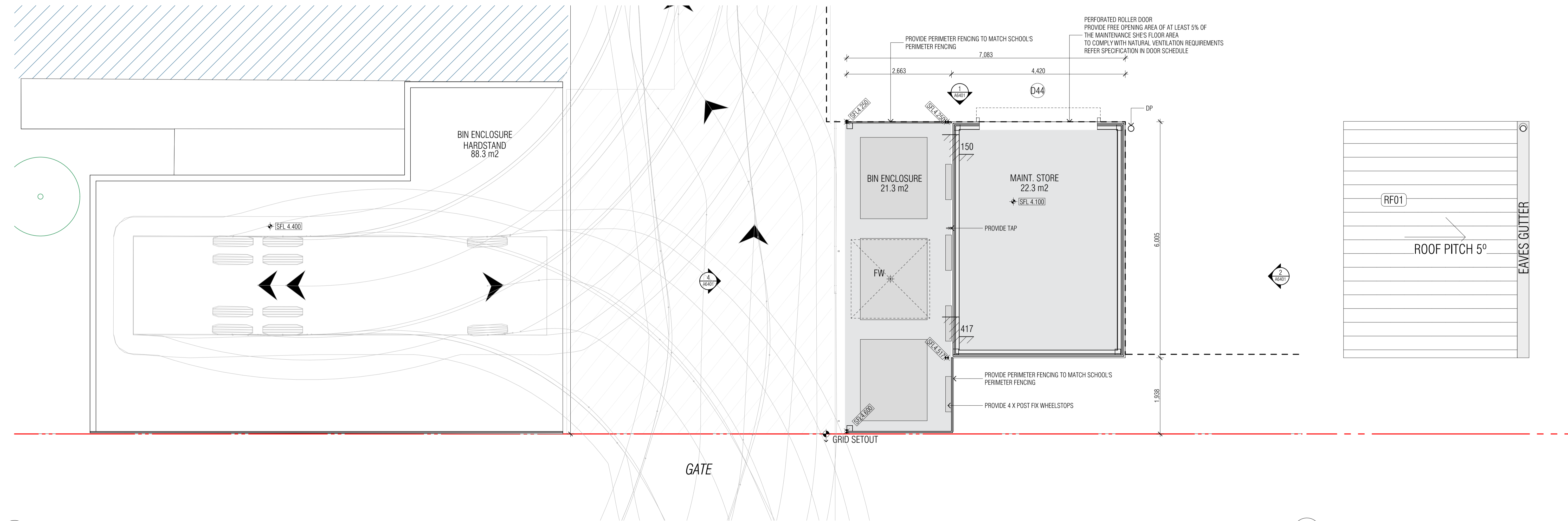
BIN ENCLOSURE PLAN SCALE 1:50@A1
