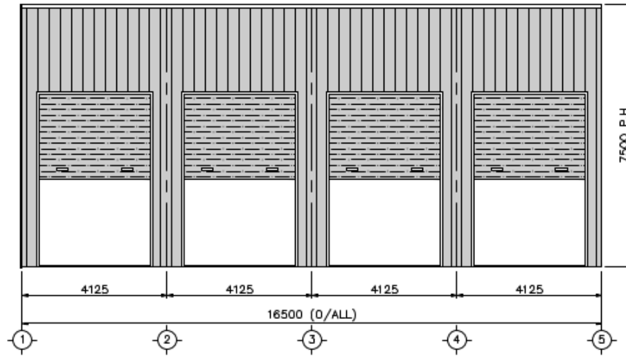
GRID B ELEVATION
