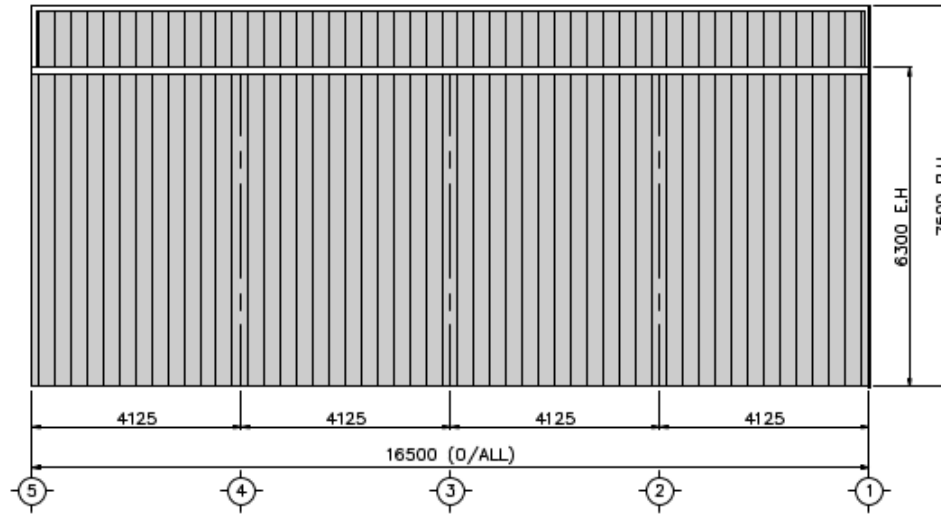
GRID A ELEVATION
