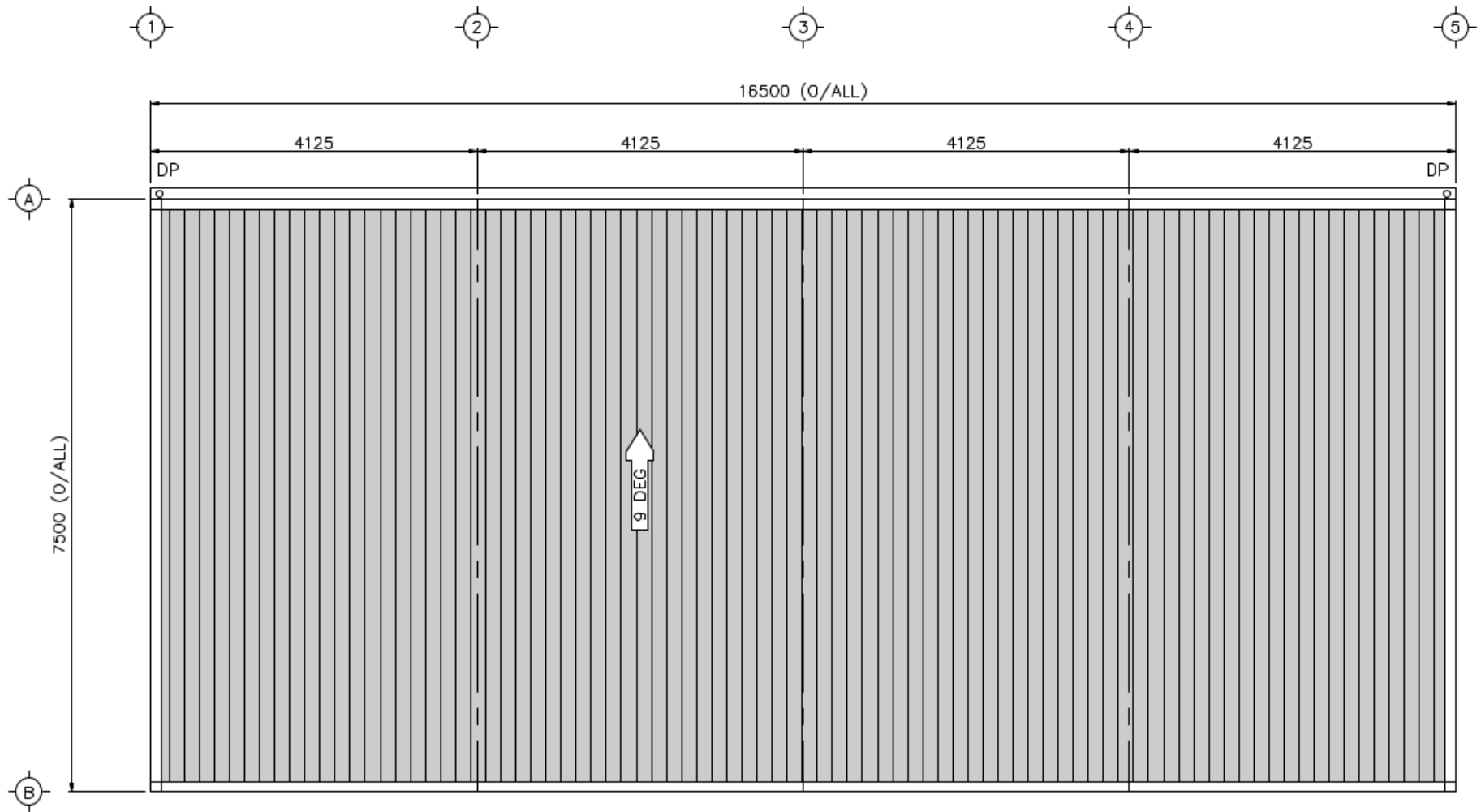
ROOF SHEETING PLAN
