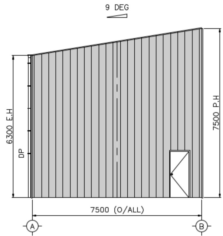
GRID 1 ELEVATION
