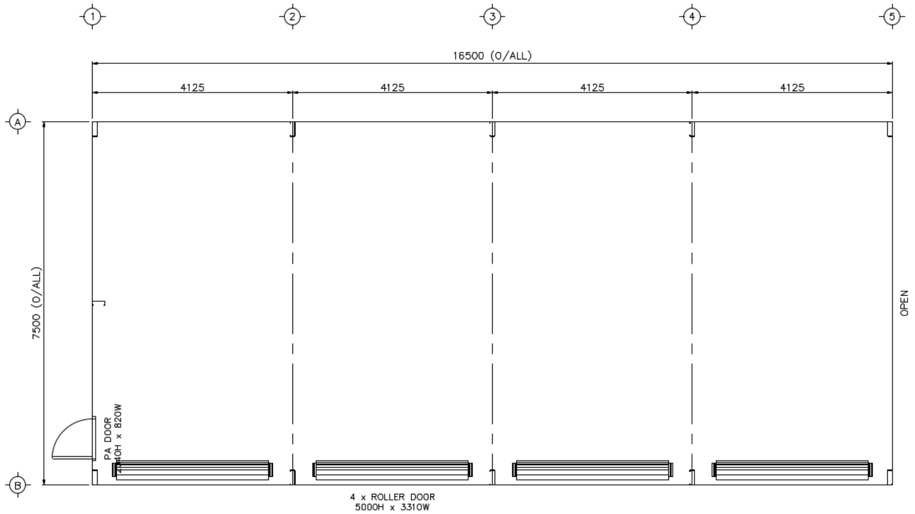
FLOOR PLAN
