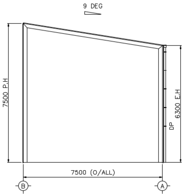
GRID 5 ELEVATION
