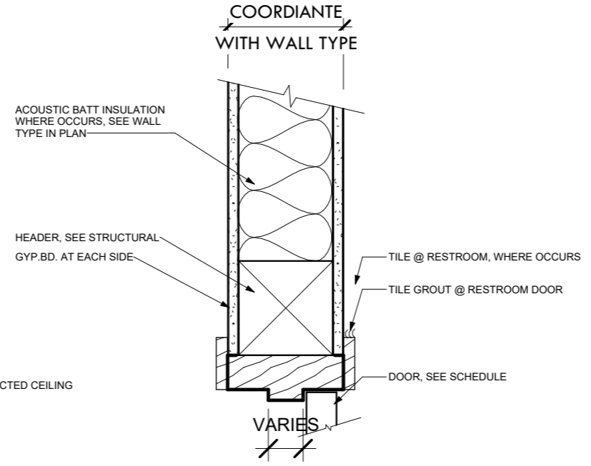
INTERIOR DOOR HEADER @ WOOD STUD
