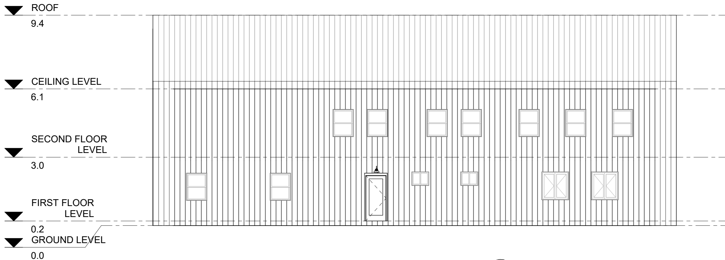
LEFT ELEVATION
