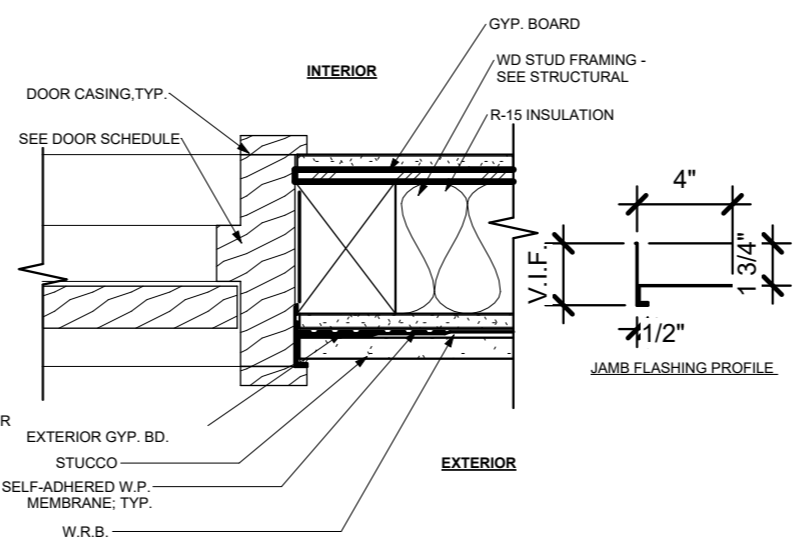
EXTERIOR DOOR JAMB_STUCCO
