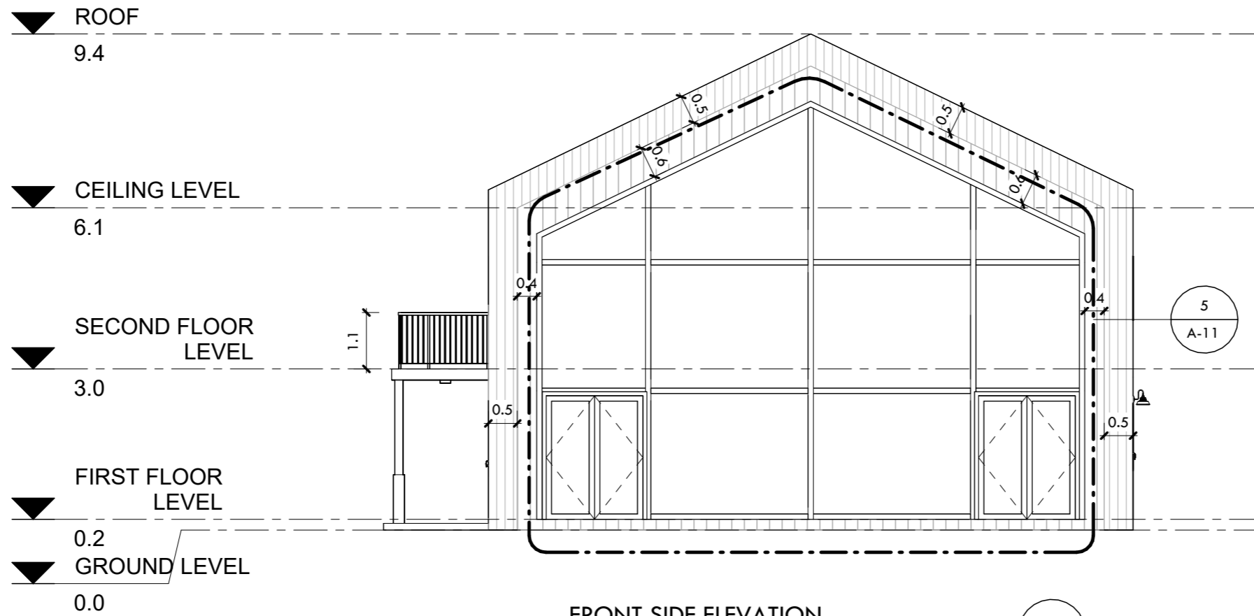
FRONT SIDE ELEVATION Scale: 1 : 100
