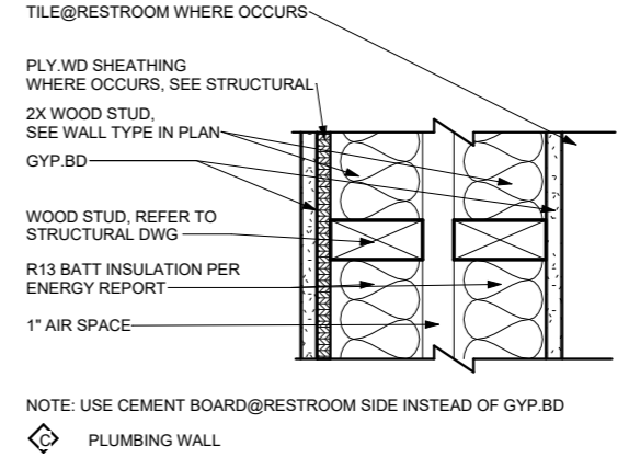
INTERIOR PLUMBING WALL
