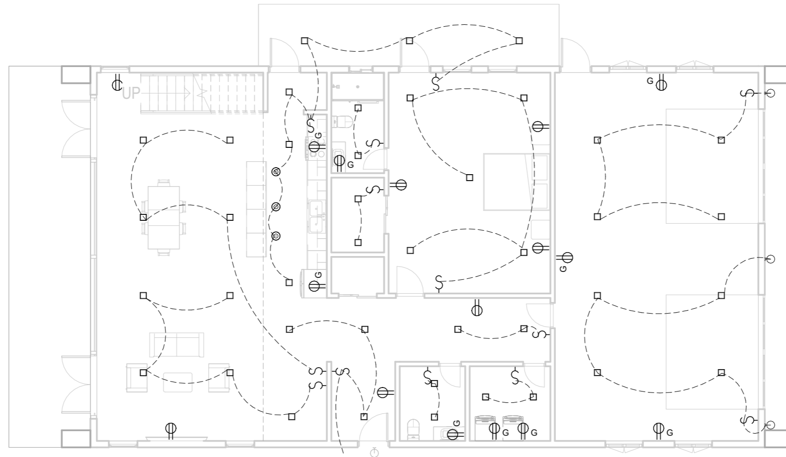
FIRST FLOOR ELECTRICAL PLAN
