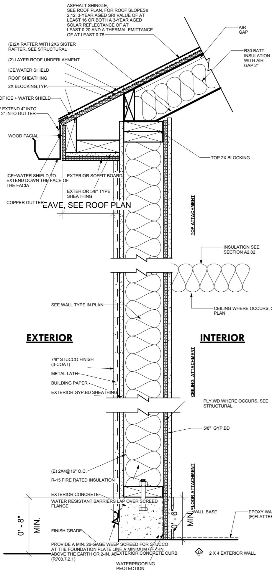
EXTERIOR WALL SECTION WITH EAVE
