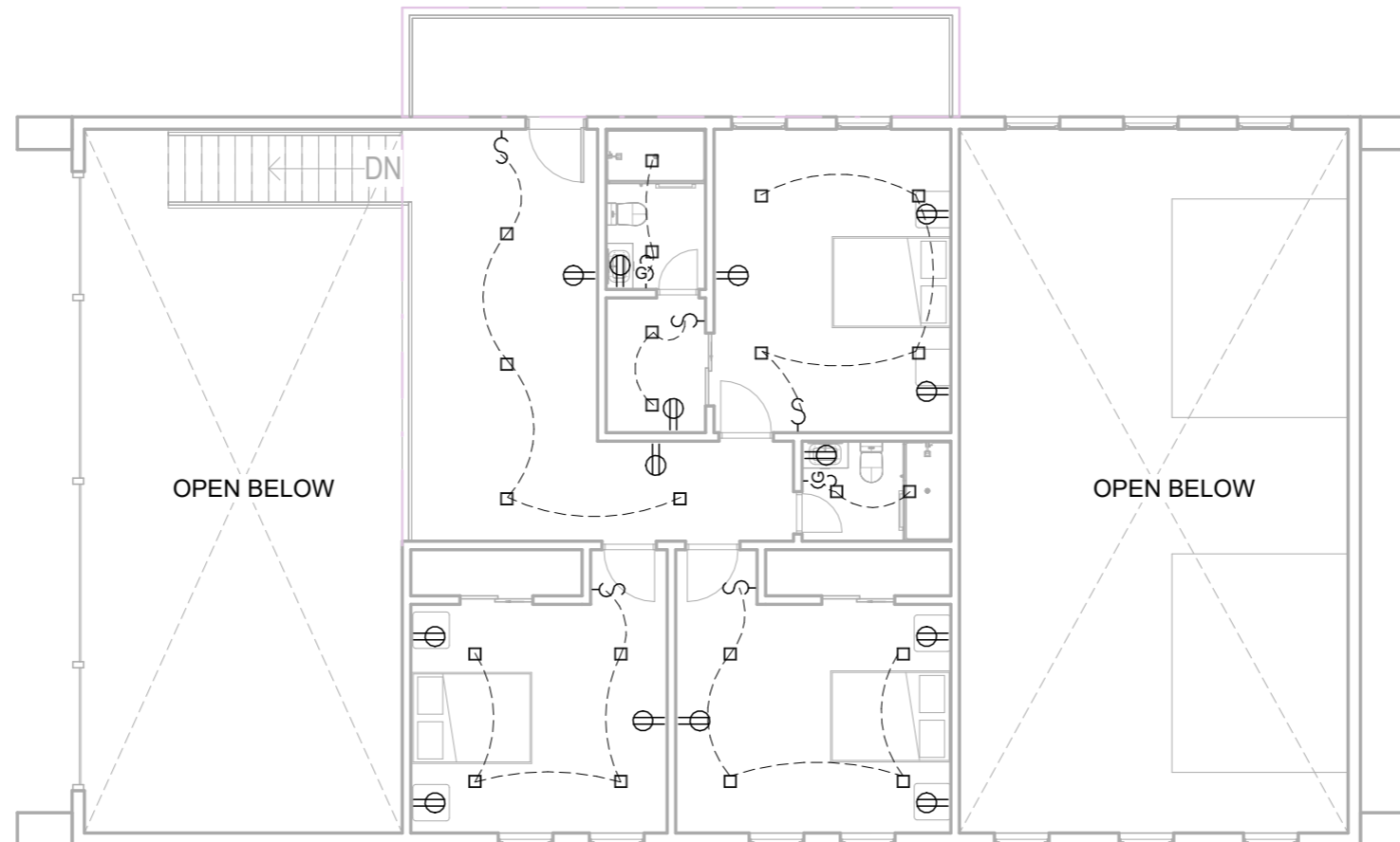
LOFT ELECTRICAL PLAN
