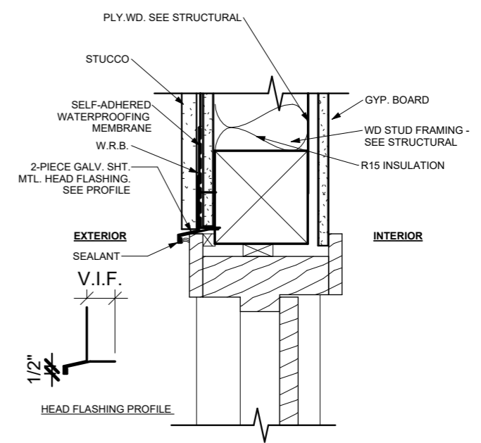
EXTERIOR DOOR HEAD_STUCCO
