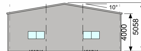
ELEVATION GRID 6
