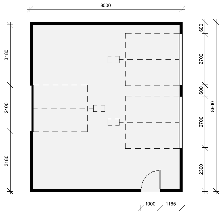
Shed Floor Plan 1 : 100
