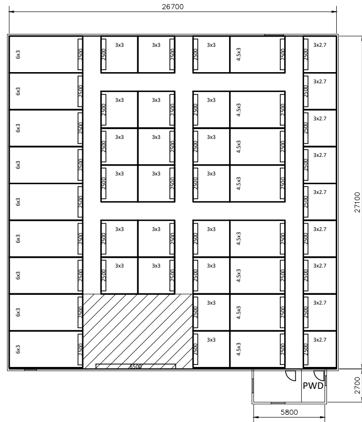
GROUND FLOOR - UNIT PLAN SCALE 1:300
