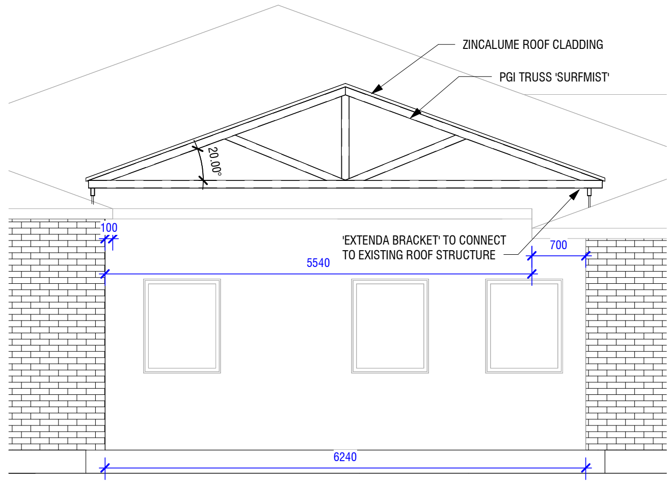
2 Elevation- Front (West) A150 1:50
