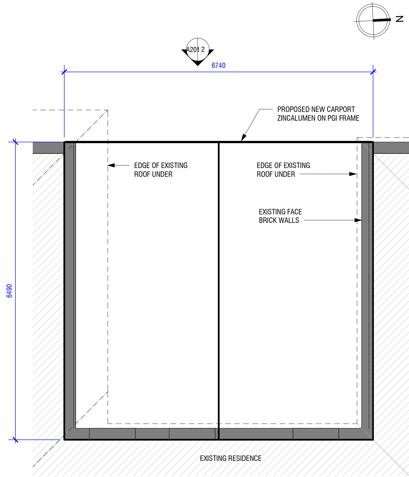
1 PLAN A101 1:50
