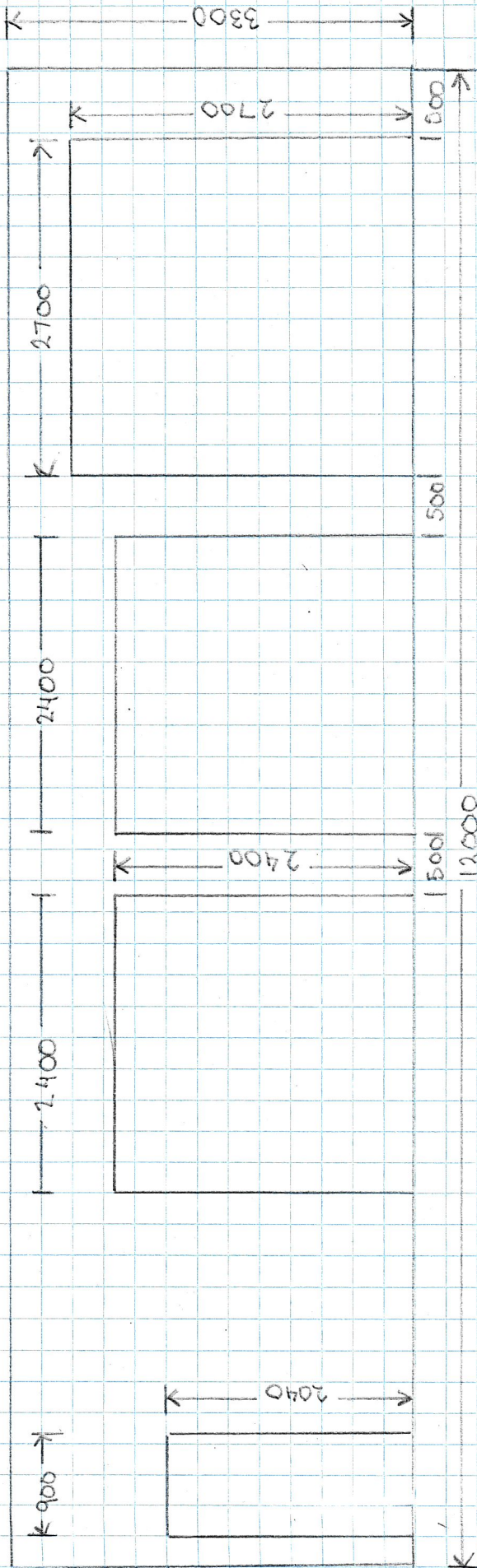
Front Elevation
